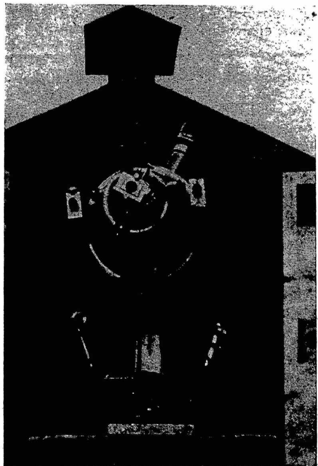
Astronominis instrumentas azimutui surasti
